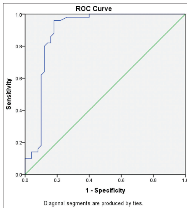
Figure 1: Receiver operating characteristic curve is between Ca/Mg ratio of cases and controls.
